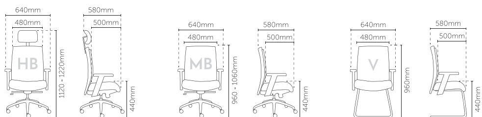
ADJUSTABLE HEADREST
